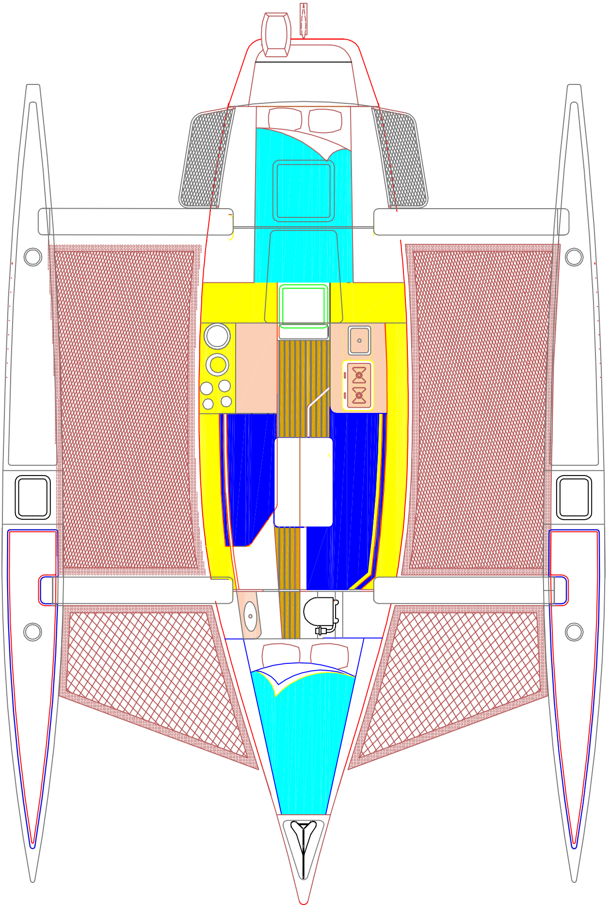
— ACCOMMODATION PLAN — Corsair Cruze 970
